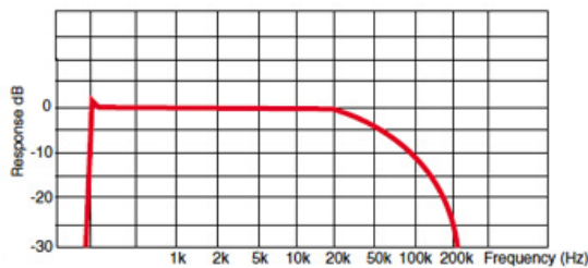
Frequency Characteristics for L-4E6S (100m)
