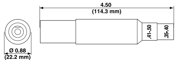
Female Plug – Set Screw
