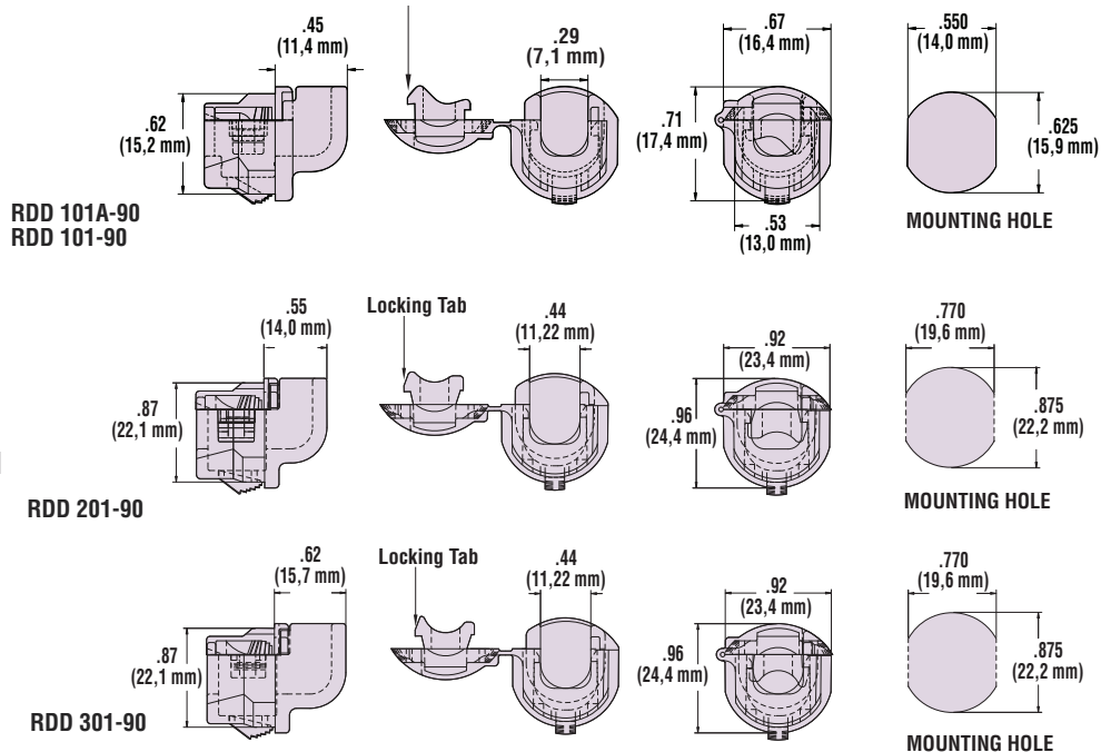
Locking Tab varies with Cable Size
