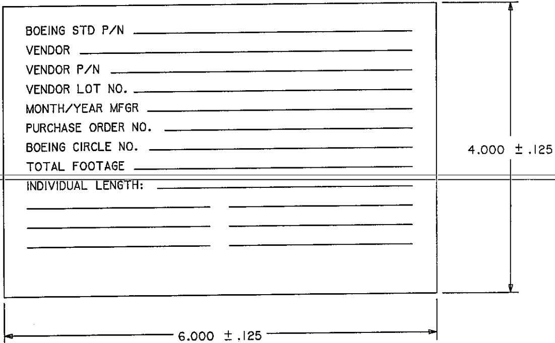
Figure 2 - Reel Label
