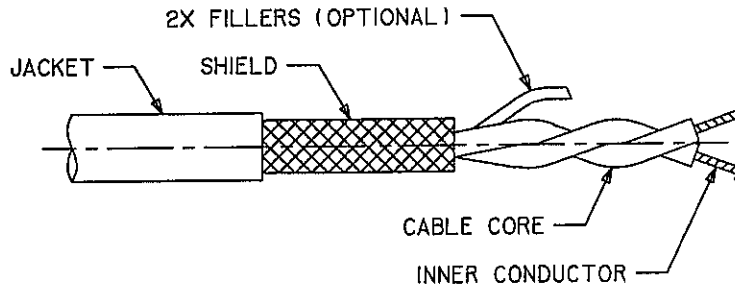
Figure 1 - Physical Configuration
