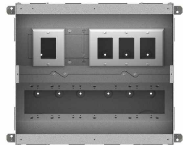
Plate Configuration 1-3 (a)
