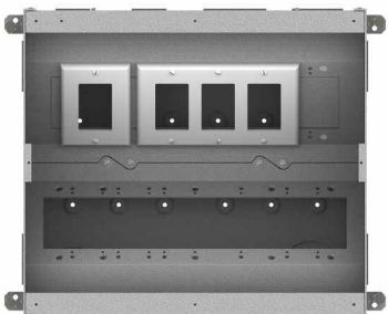
Plate Configuration 1-3 (b)
