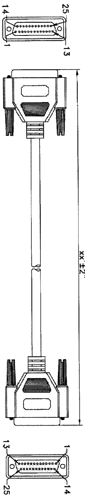
FRONT VIEW DB25 FEMALE DB25 FEMALE FRONT VIEW
