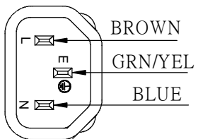
IEC-60320-C14
