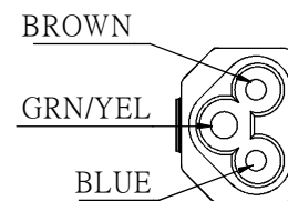
IEC-60320-C5
