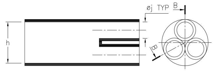
SECTION B-B
