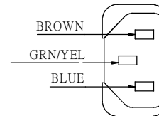
IEC-60320-C13
