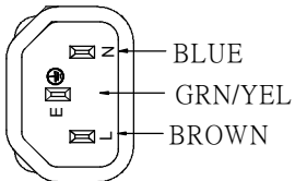
IEC-60320-C14
