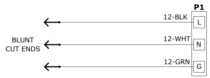
WIRING DIAGRAM
