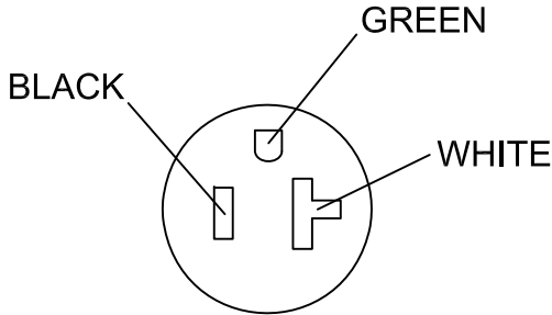
WIRING DETAIL-FEMALE
