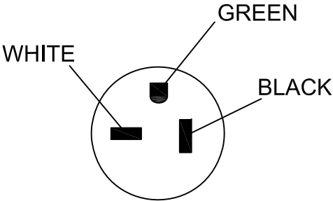
WIRING DETAIL-MALE
