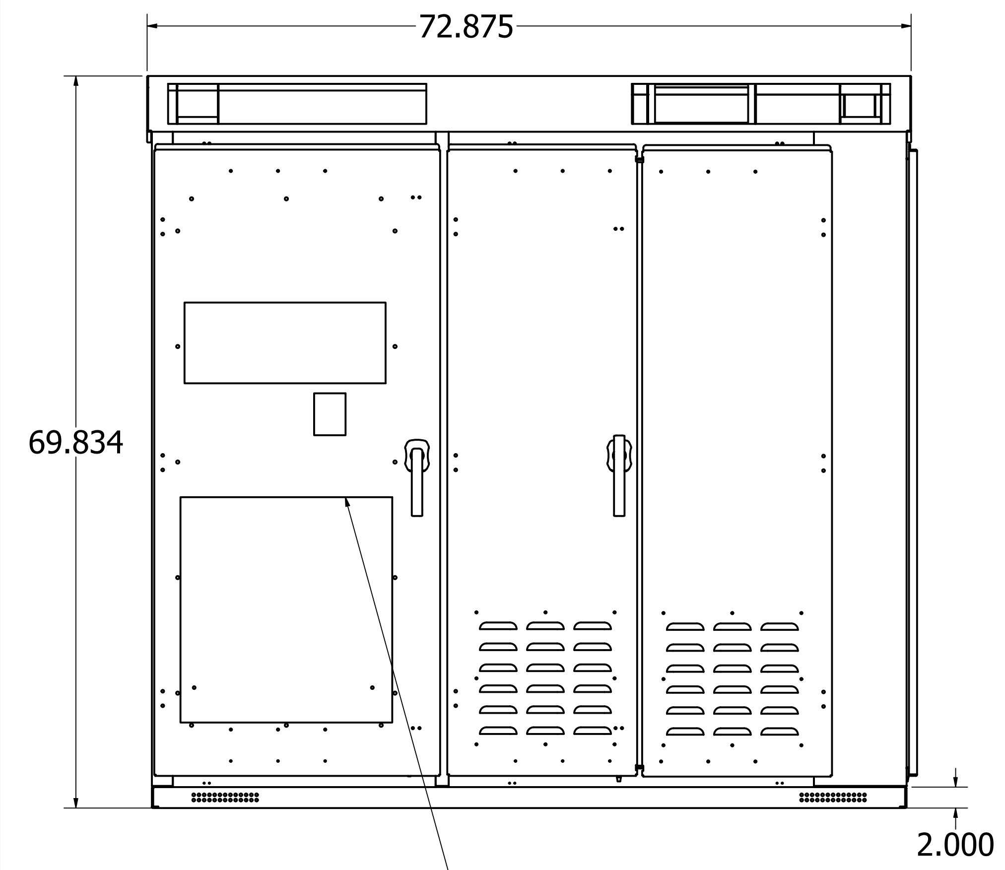
FRONT VIEW (WITH FANHOOD & PLINTH)
