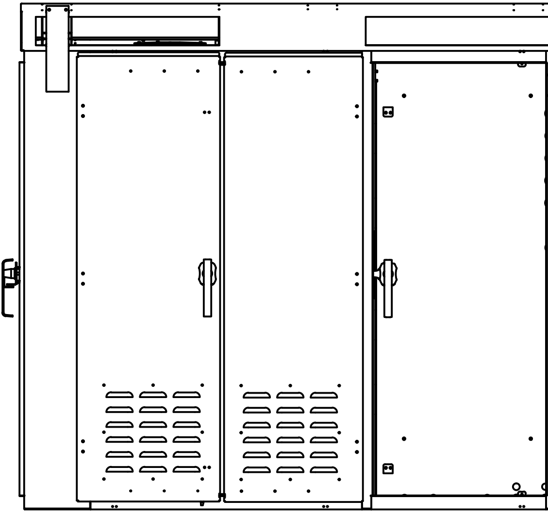
REAR VIEW BACK BATTERY DOOR REMOVED
