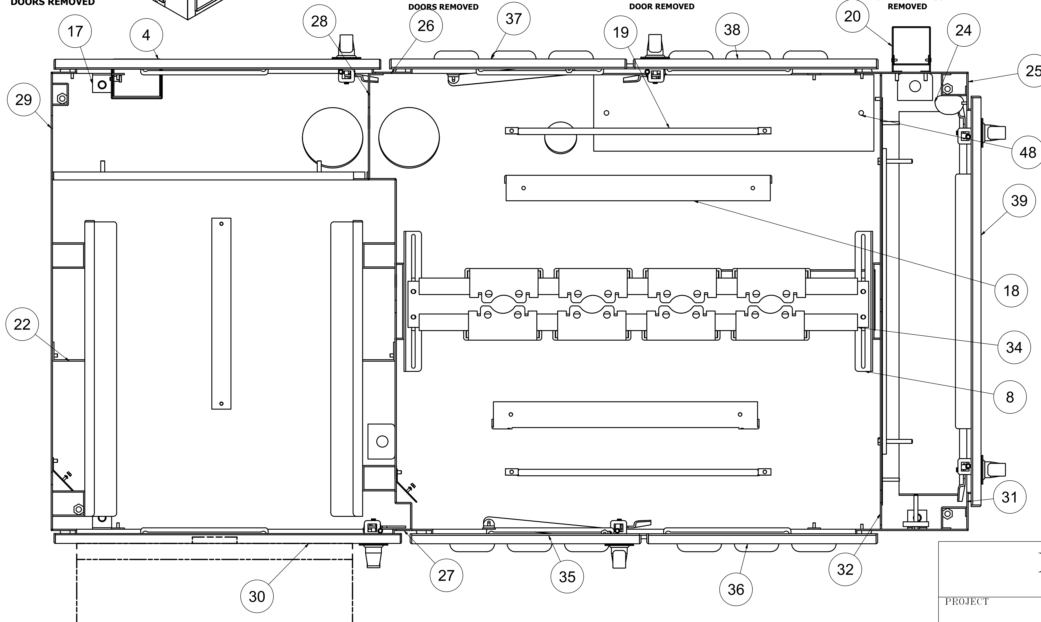
TOP VIEW FANHOOD & TOP REMOVED
