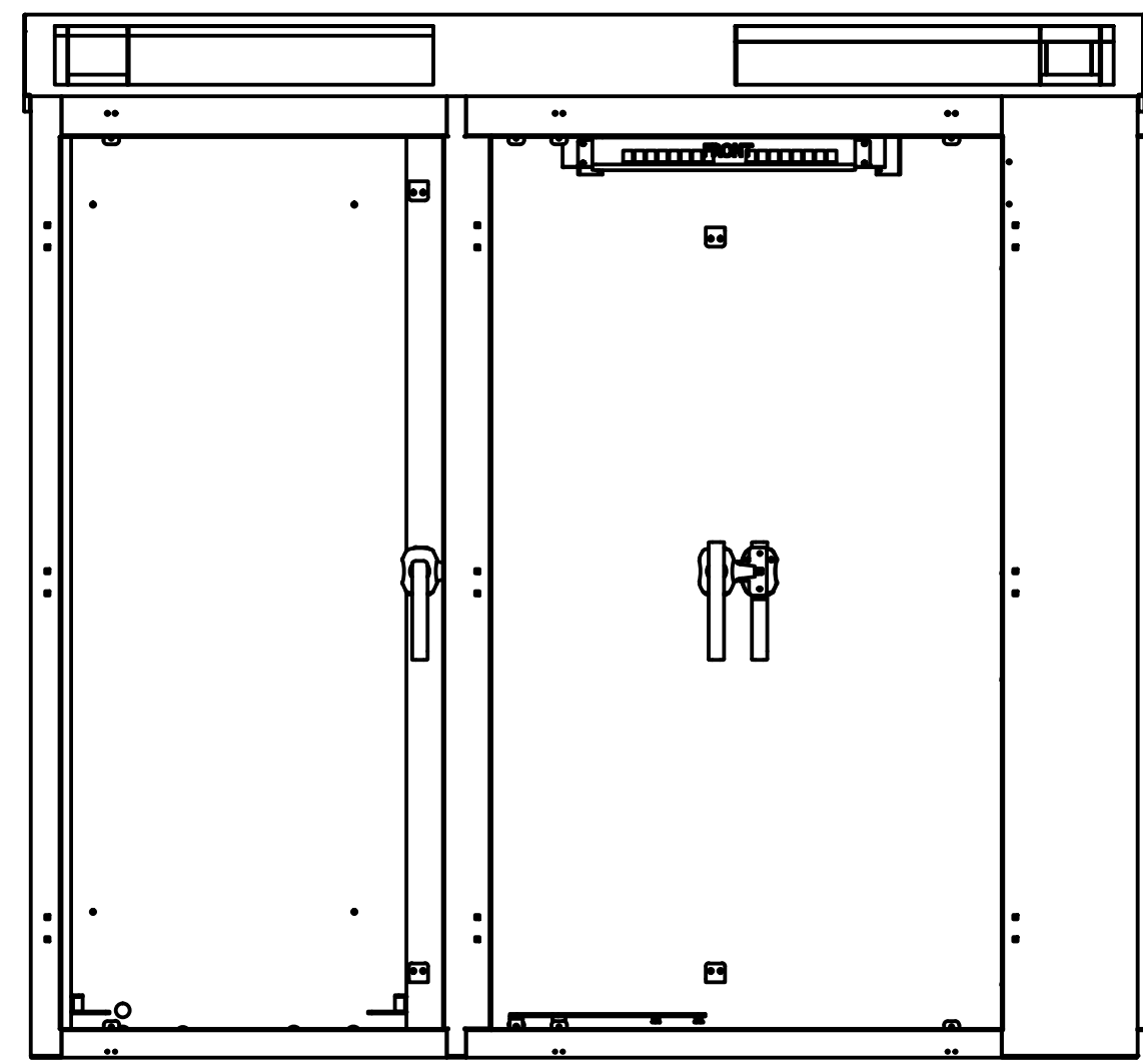
FRONT VIEW DOORS REMOVED
