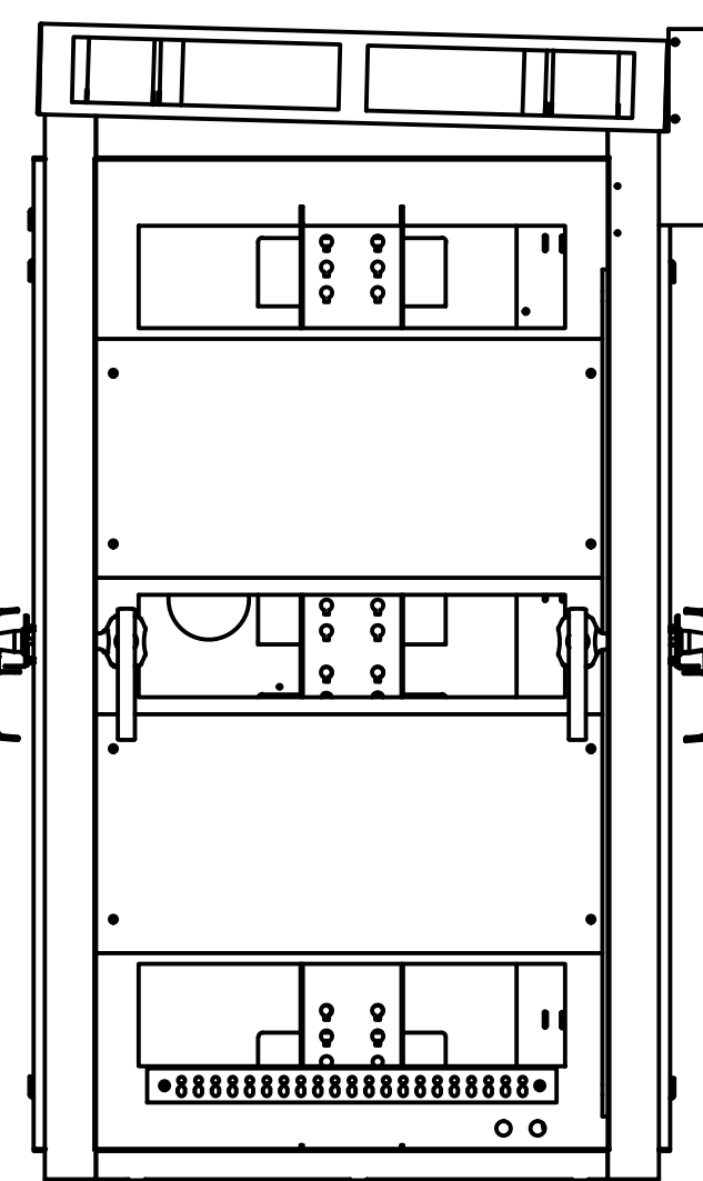
RIGHT SIDE VIEW DOOR REMOVED
