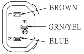
IEC-60320-C14
