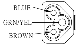
IEC-60320-C5
