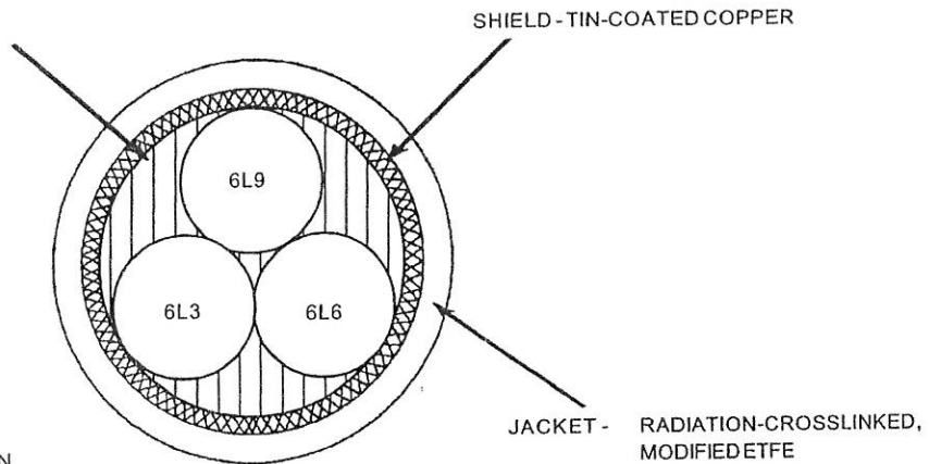
CABLE CONSTRUCTION DETAILS
