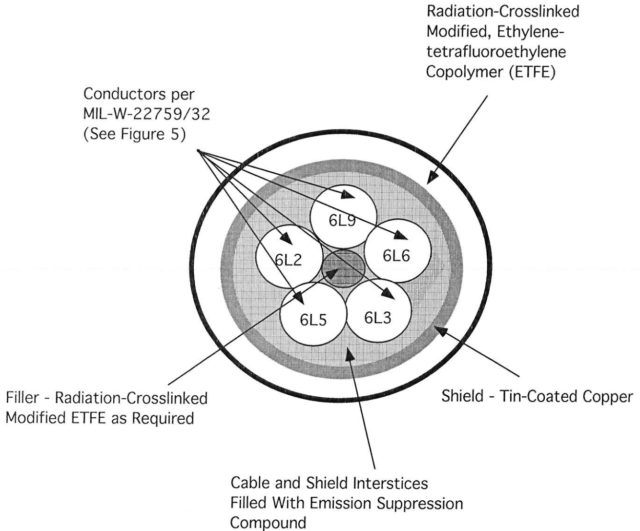
FIGURE 4 - CABLE CONSTRUCTION DETAILS (FIVE CONDUCTORS)
