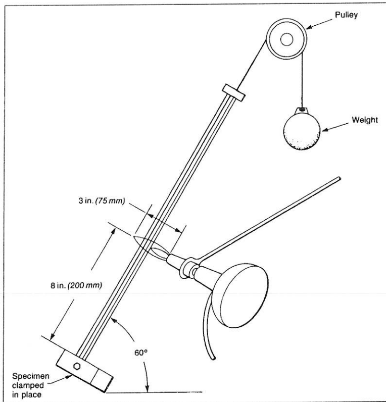
Figure 1. Flammability Test Apparatus, Procedure 1 (shown without chamber)
