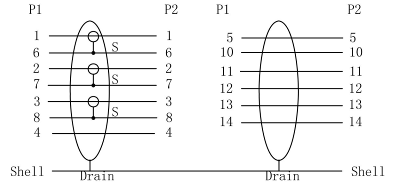
PIN Assignment
