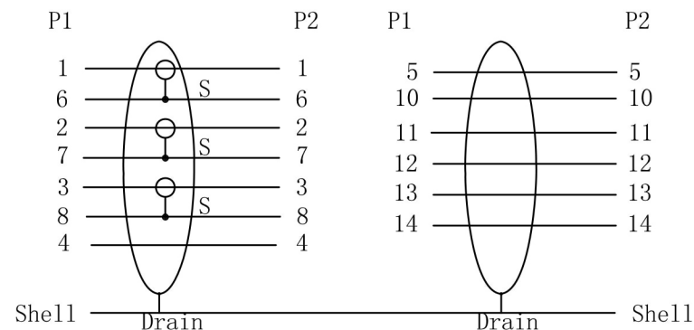
PIN Assignment
