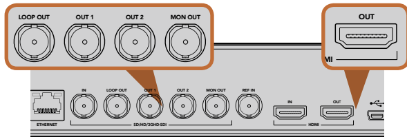
HyperDeck Studio SDI and HDMI outputs. SDI outputs include a Loop Out and a Monitor output.
