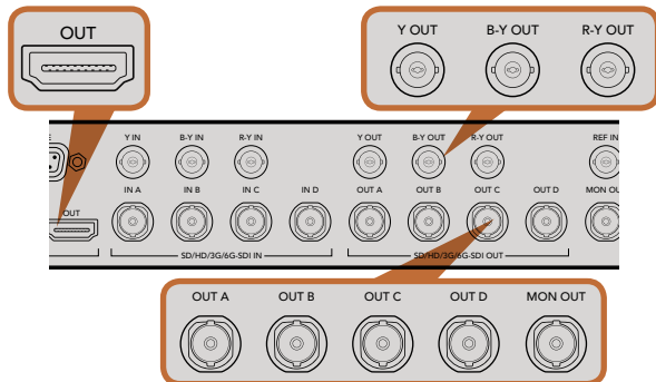
HyperDeck Studio Pro HDMI, analog component and SDI outputs plus Monitor Out.
