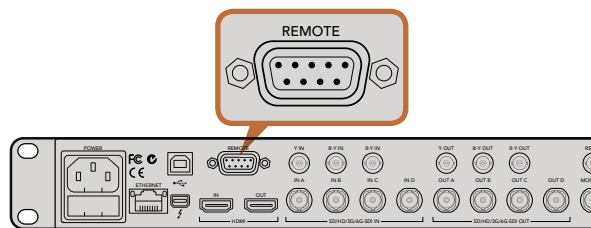
Remote port on HyperDeck Studio Pro.
