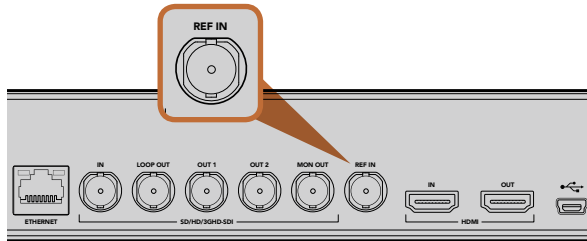
Reference input on HyperDeck Studio.
