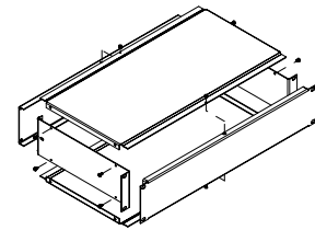
front and rear panels detach for simplified machining
