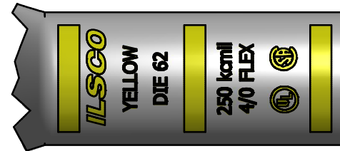
DETAIL F SCALE 2 : 1 INK MARK TOP & BOTTOM INK COLOR: YELLOW
