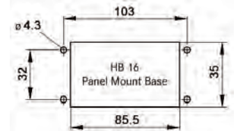
all dimensions are in mm.
