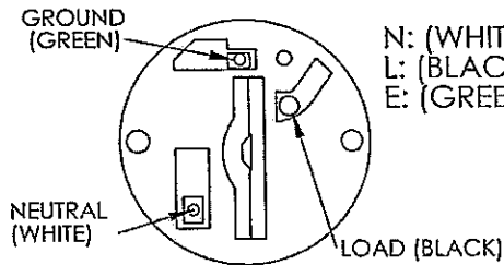
SCREW TERMINAL VIEW CONNECTOR REAR VIEW
