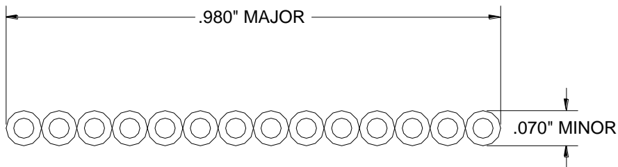
Cross Section
