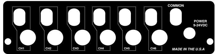
Muxing SDI Signals
