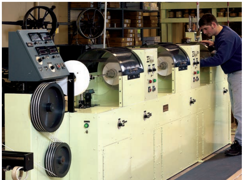
Triple Head Wrapper for PTFE tape and other films
