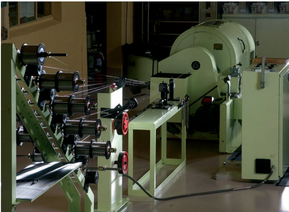
Buncher set up for stranding Resistance Wire
