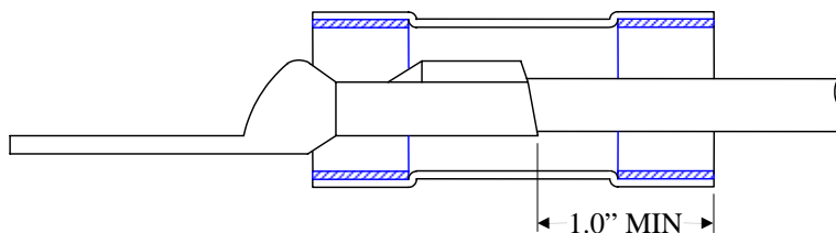
Figure 1. RT-555 sealing sleeve location on terminals
