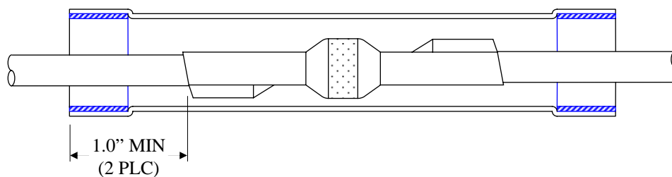
Figure 2. RT-555 sealing sleeve location on in-line splices
