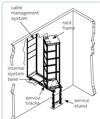
AX-SXR rotating slide out rack (for detailed millwork specifications refer to A&E #96-0100)
