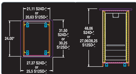
12 and 24 space isolation rack top view front view
