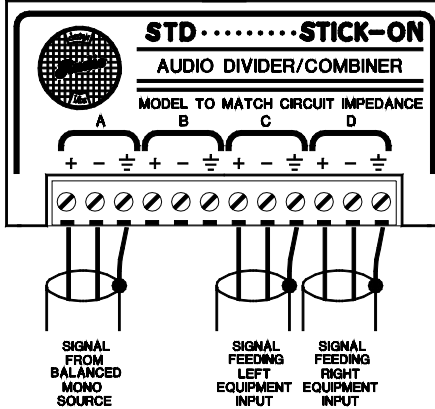
FEED MONO SIGNALS TO STEREO INPUTS
