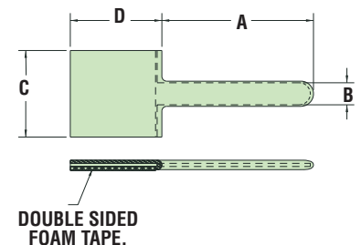
VCSC ADHESIVE BACK MOUNT
