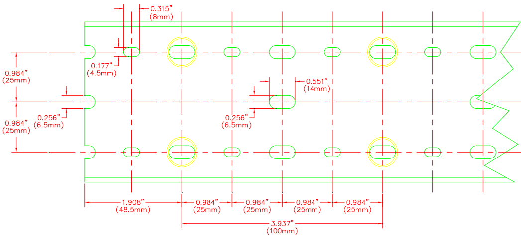
BASE PERFORATION
