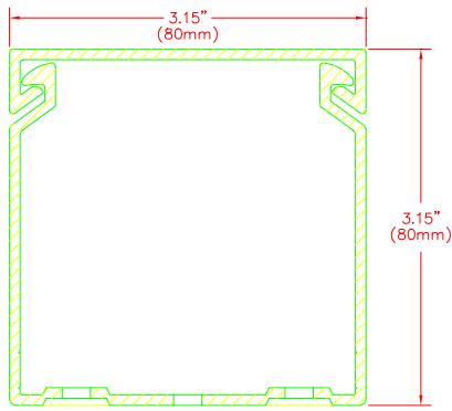
FRONT SECTION
