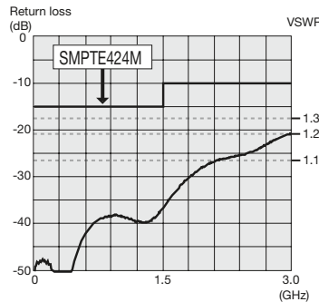
Fig. 1 Return loss for BCP-C3B
