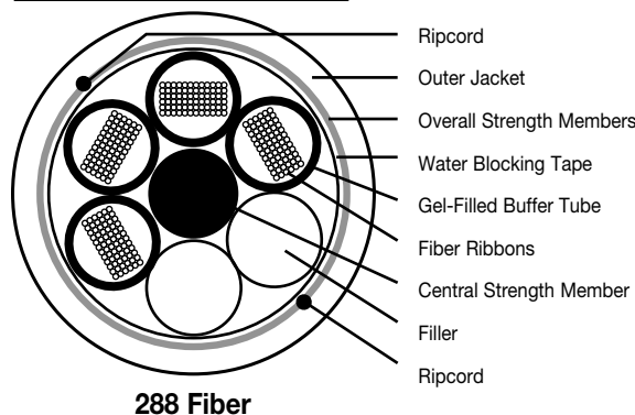
288 Fiber
