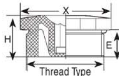
Nylon Hex Plug
